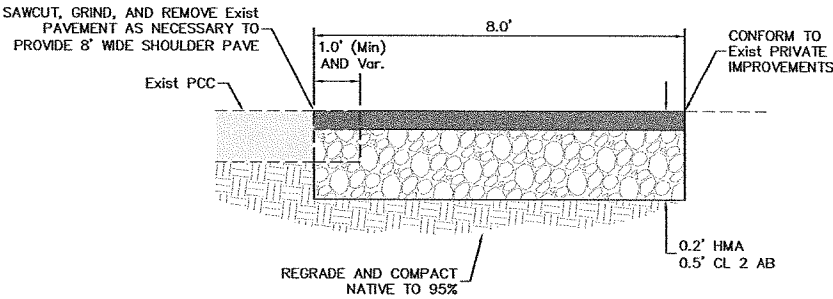
PARKING SECTION (SAN CARLOS AVE) NTS
