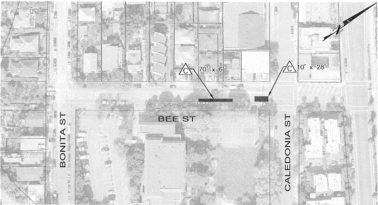
SECTION 13: BEE STREET (BONITA ST TO CALEDONIA ST) TREATMENT: PCC FAILURE REPAIR
